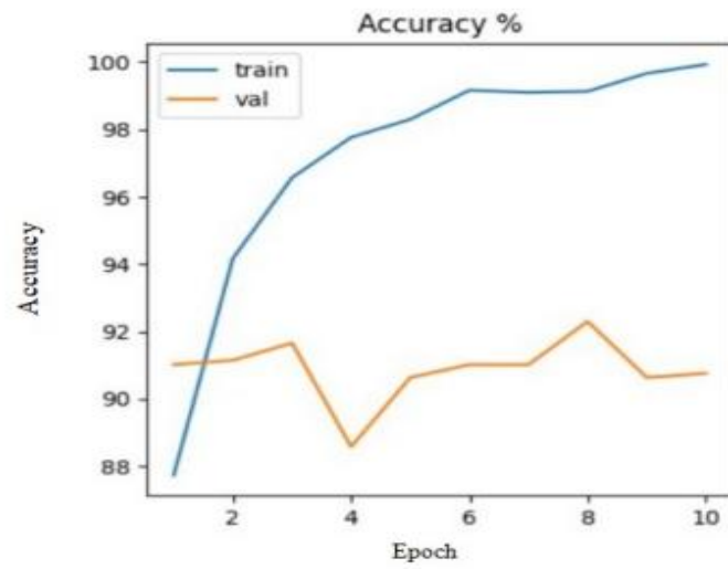
Fig. 5. Training and Validation Accuracy over Epochs
