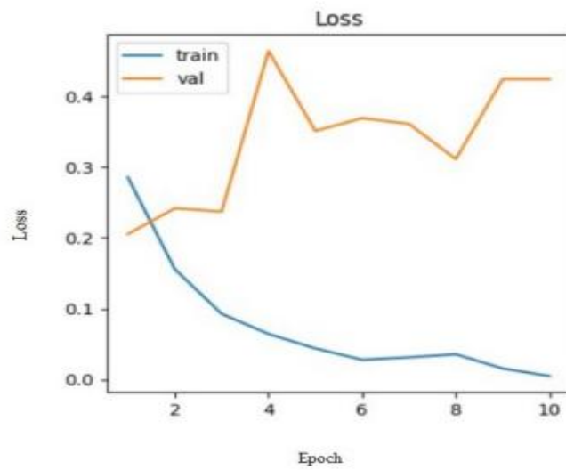
Fig. 6. Training and Validation Loss over Epochs
